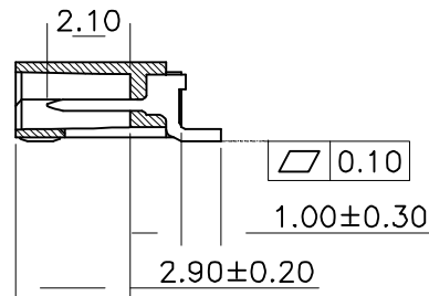
X-X SEC
