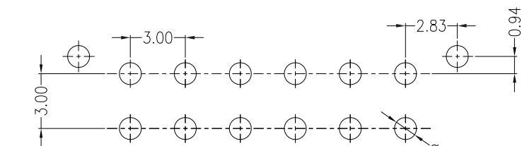
SUGGESTED PCB LAYOUT
